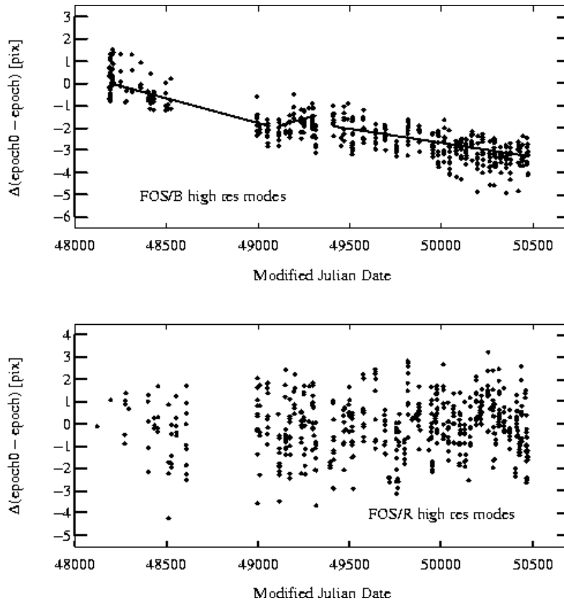
Figure 1: Measured cross-correlation offset in pixels between individual WAVECALs and pipeline-defining epoch WAVECAL. Upper panel: FOS/BL high-resolution dispersers. Lower panel: FOS/RD high-resolution dispersers.
