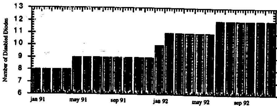
Figure 3.1b: FOS Red Detector Disabled Diode History
