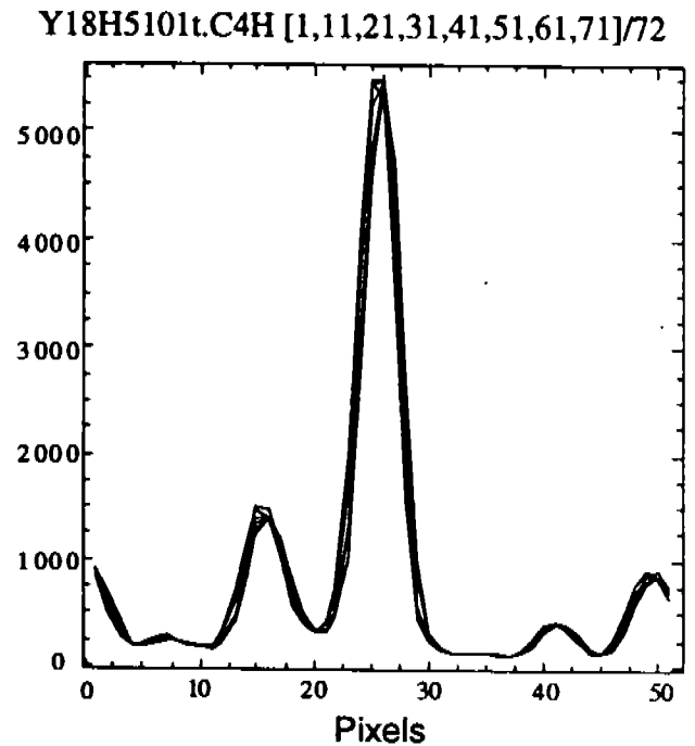
Figure 3.5b: Single line spread, 2880 Sec Red Detector with GIMP correction
