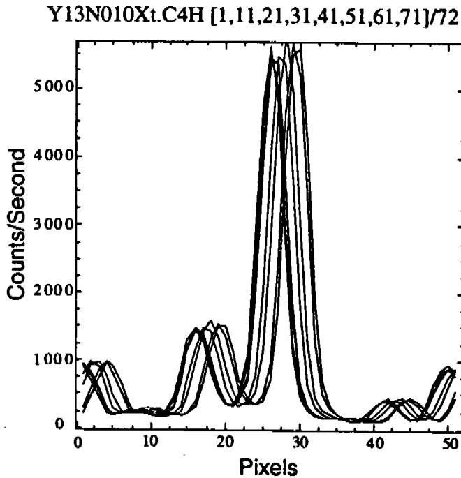
Figure 3.5a: Single line spread, 2880 Sec Red Detector No GIMP correction
